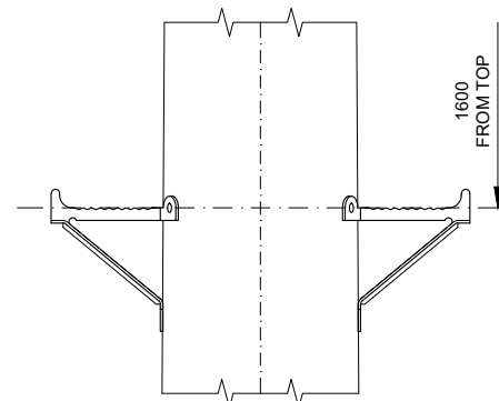
DETAIL D - ANTENNA ACCESS CLIMBING STEP Scale 1:10
