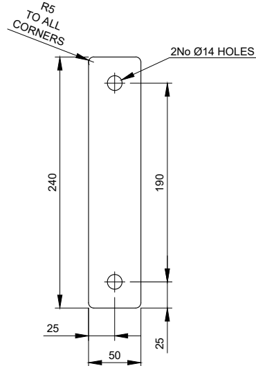
TPB-C-1 - 10mm THICK Scale 1:5
