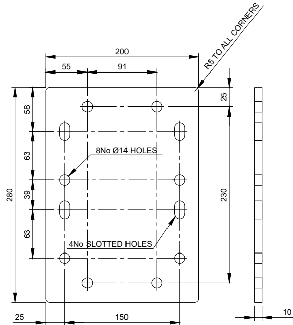
TPA-C - 10mm THICK Scale 1:5
