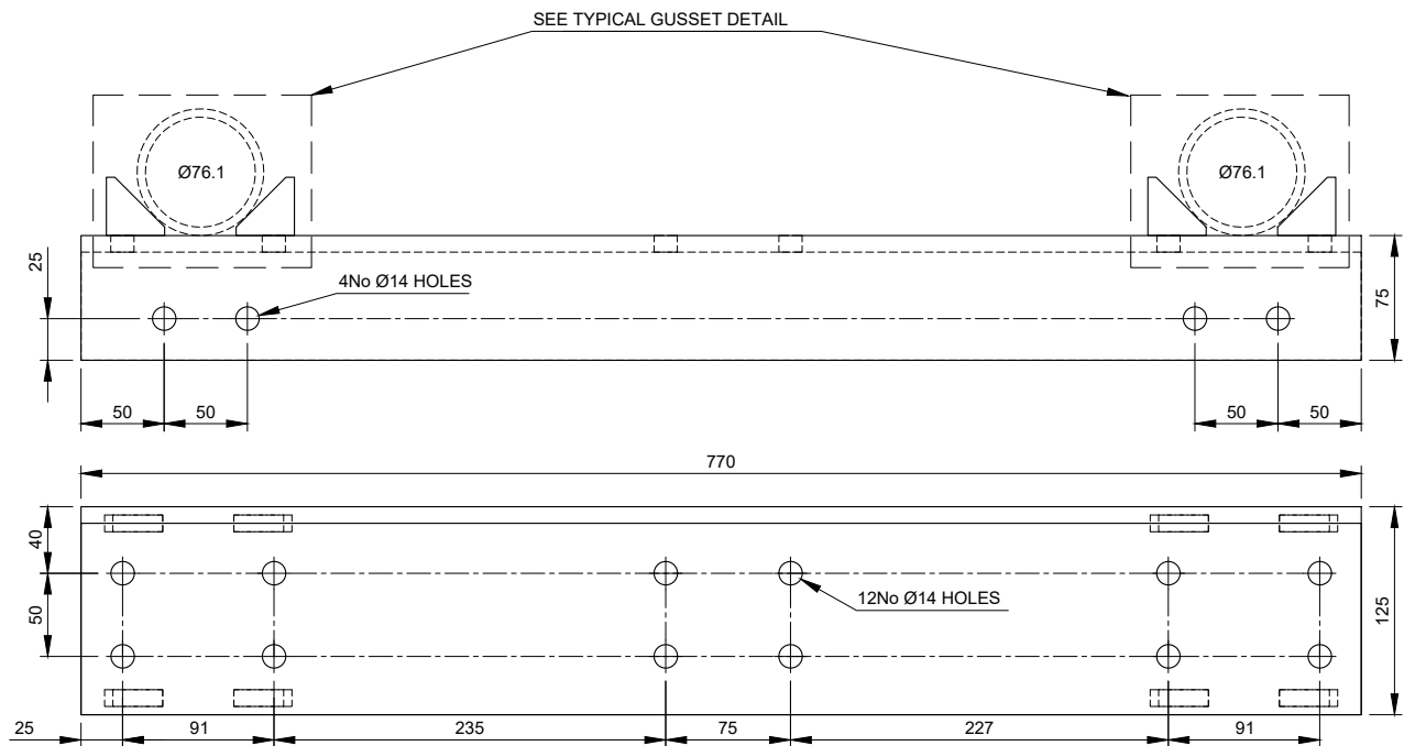
TPA-A - UA125x75x10 Scale 1:5
