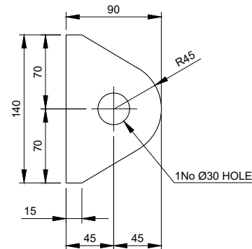
TPB-C-2 - 10mm THICK Scale 1:5
