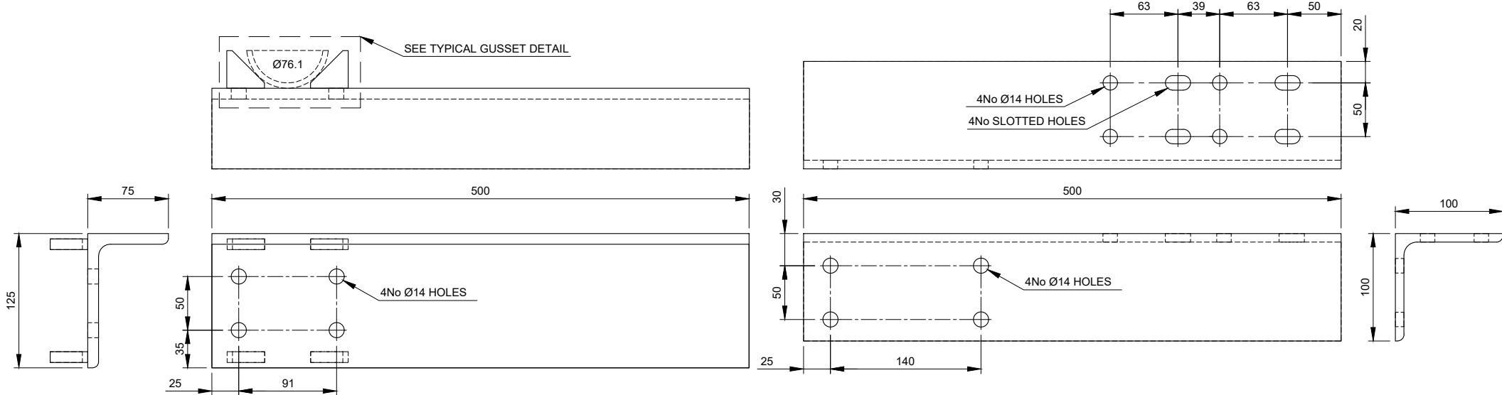
TPA-B-1 - EA100x100x8 Scale 1:5
