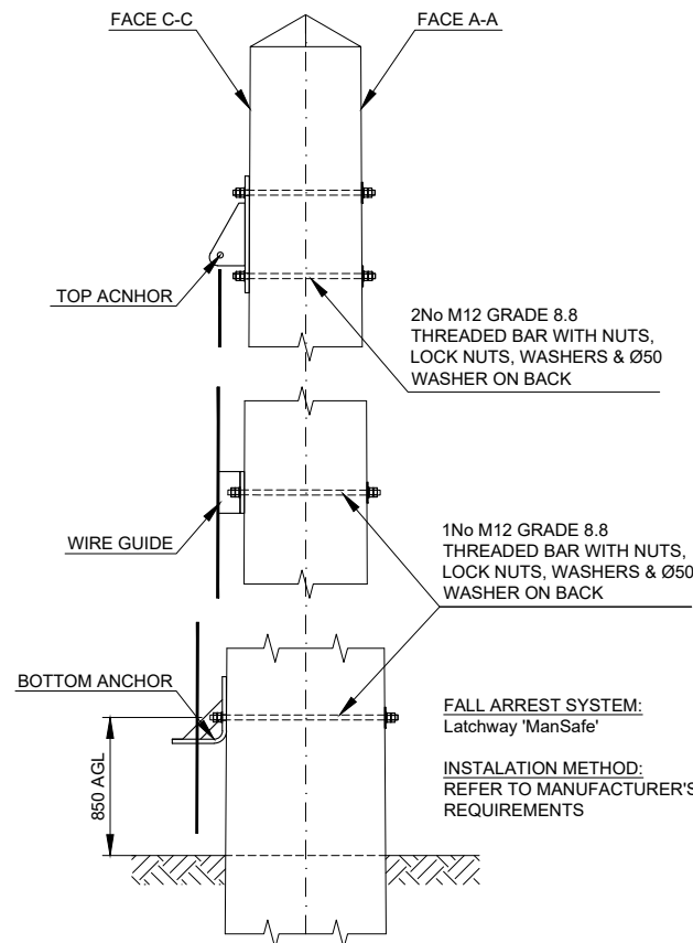
DETAIL B - FALL ARREST SYSTEM Scale 1:20
