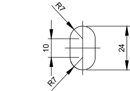
SLOTTED HOLE DETAIL Scale 1:2
